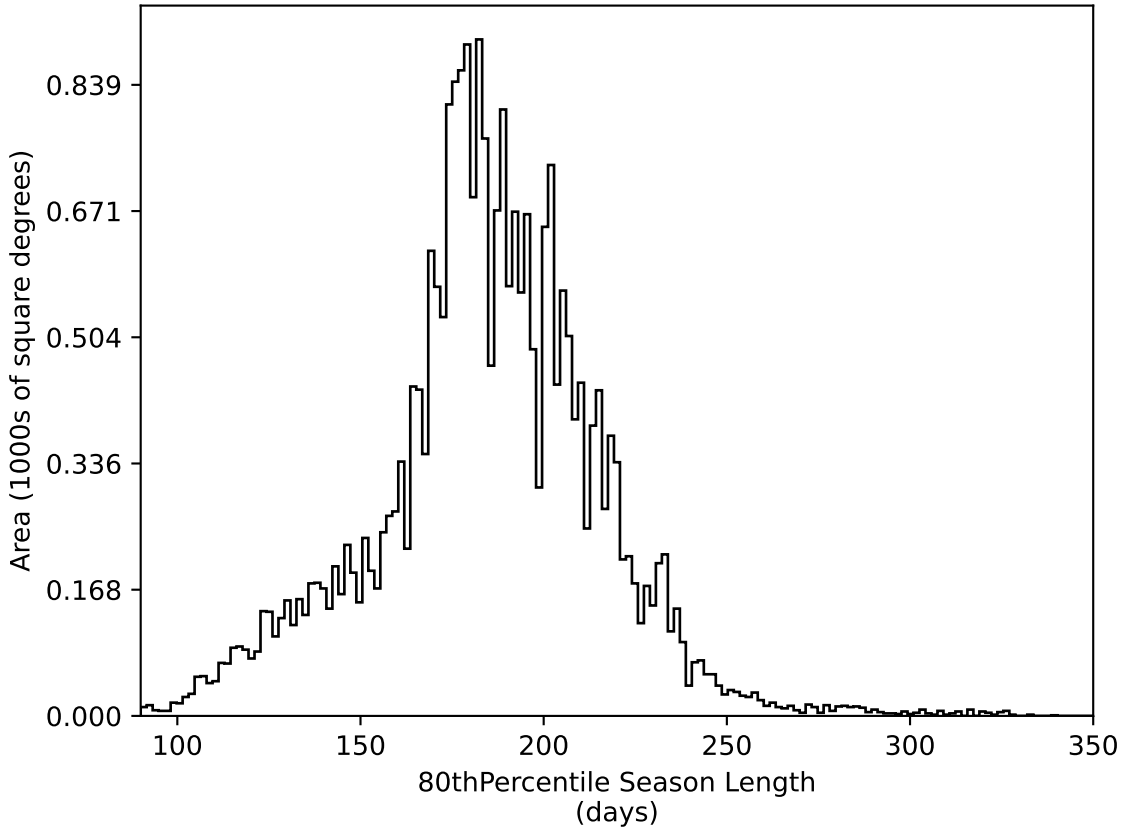
too_5_1v3.4_10yrs All sky all bands: 80thPercentile Season Length
