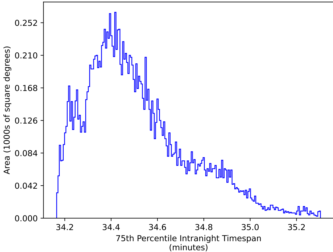
too_5_1v3.4_10yrs WFD zy bands: 75th Percentile Intranight Timespan
