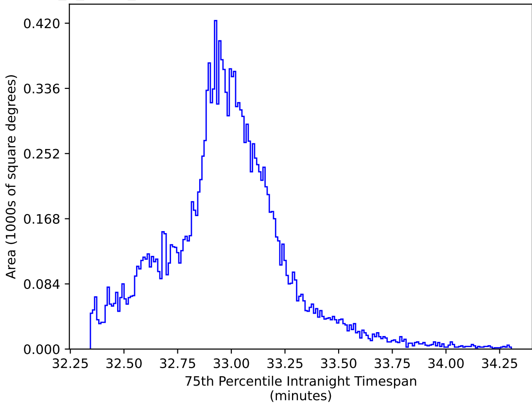
too_5_1v3.4_10yrs WFD y band: 75th Percentile Intranight Timespan
