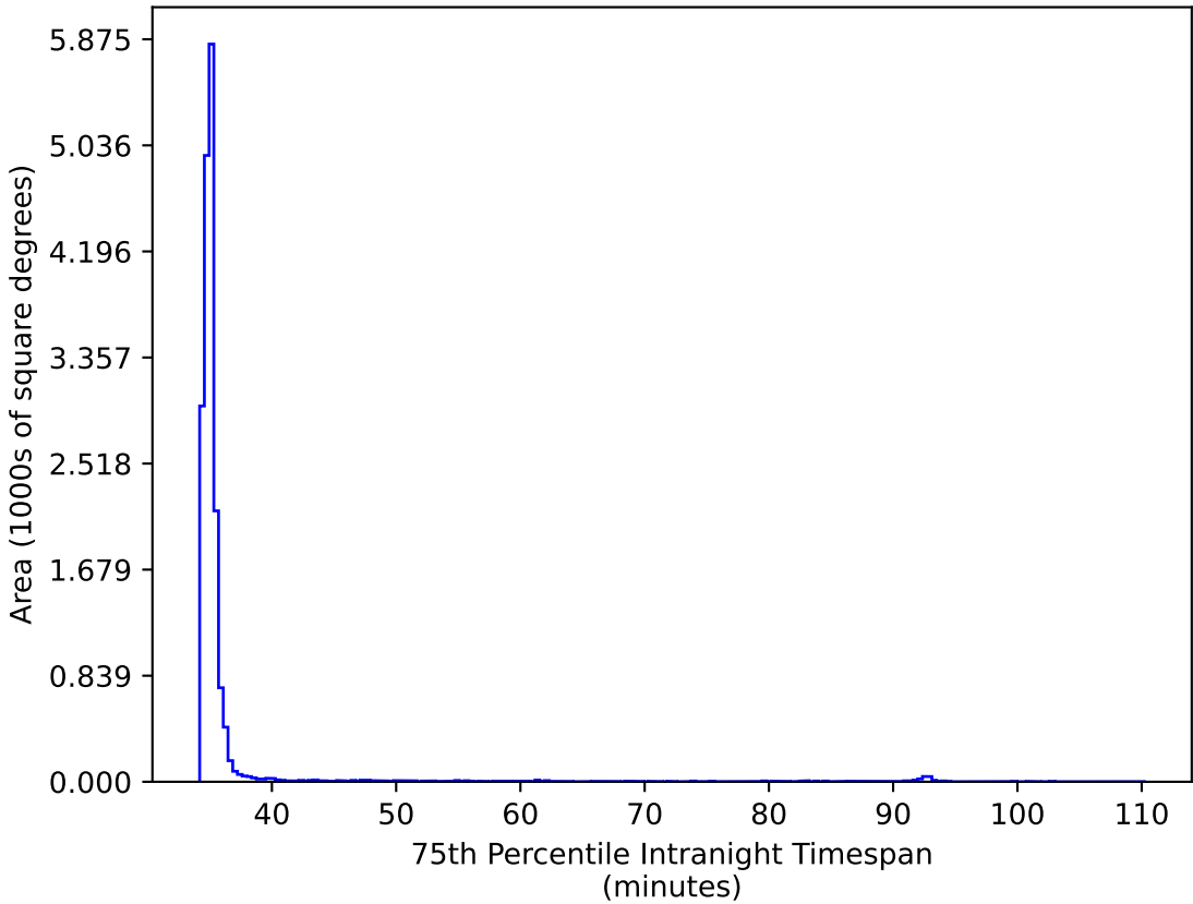
too_5_1v3.4_10yrs WFD ri bands: 75th Percentile Intranight Timespan
