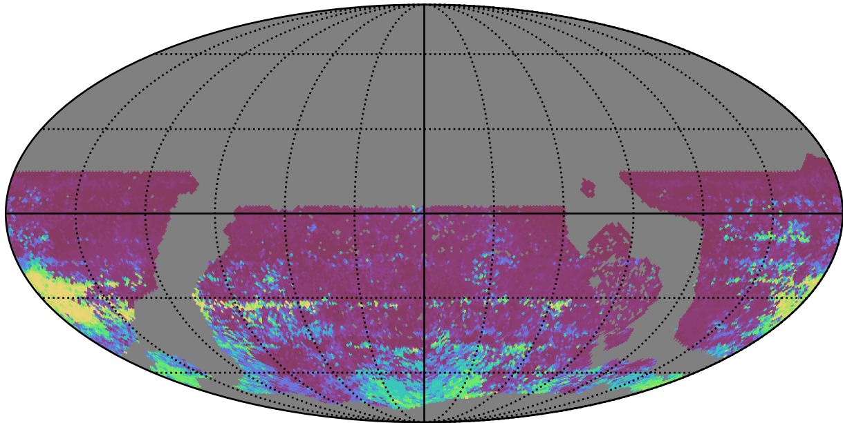
too_5_1v3.4_10yrs WFD r band: 75th Percentile Intranight Timespan
