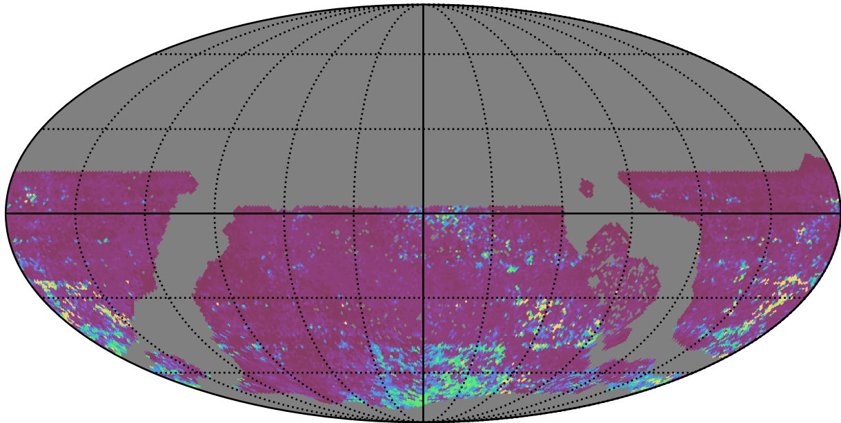
too_5_1v3.4_10yrs WFD i band: 75th Percentile Intranight Timespan
