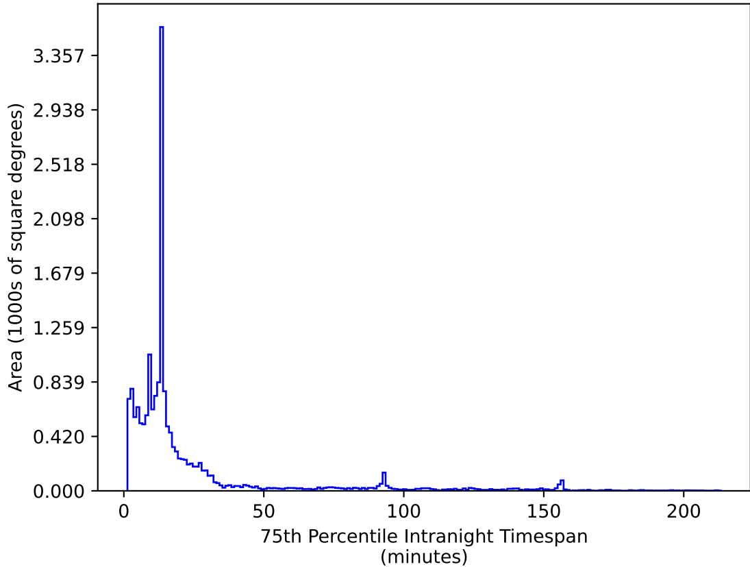
too_5_1v3.4_10yrs WFD i band: 75th Percentile Intranight Timespan
