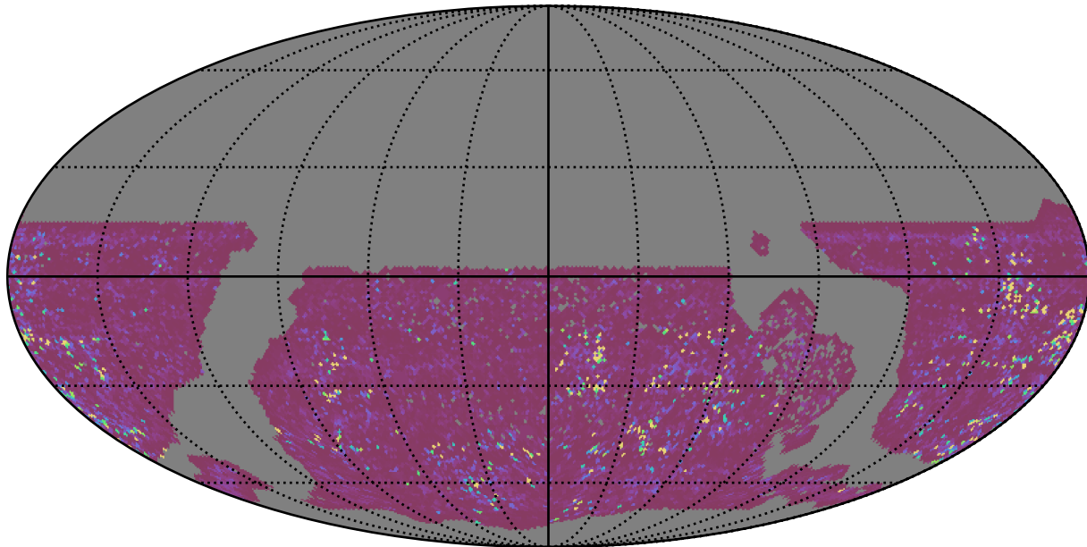
too_5_1v3.4_10yrs WFD g band: 75th Percentile Intranight Timespan
