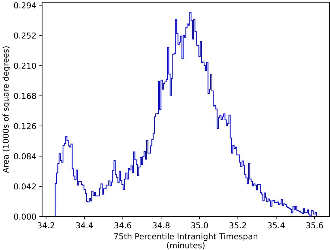
too_5_1v3.4_10yrs WFD all bands: 75th Percentile Intranight Timespan
