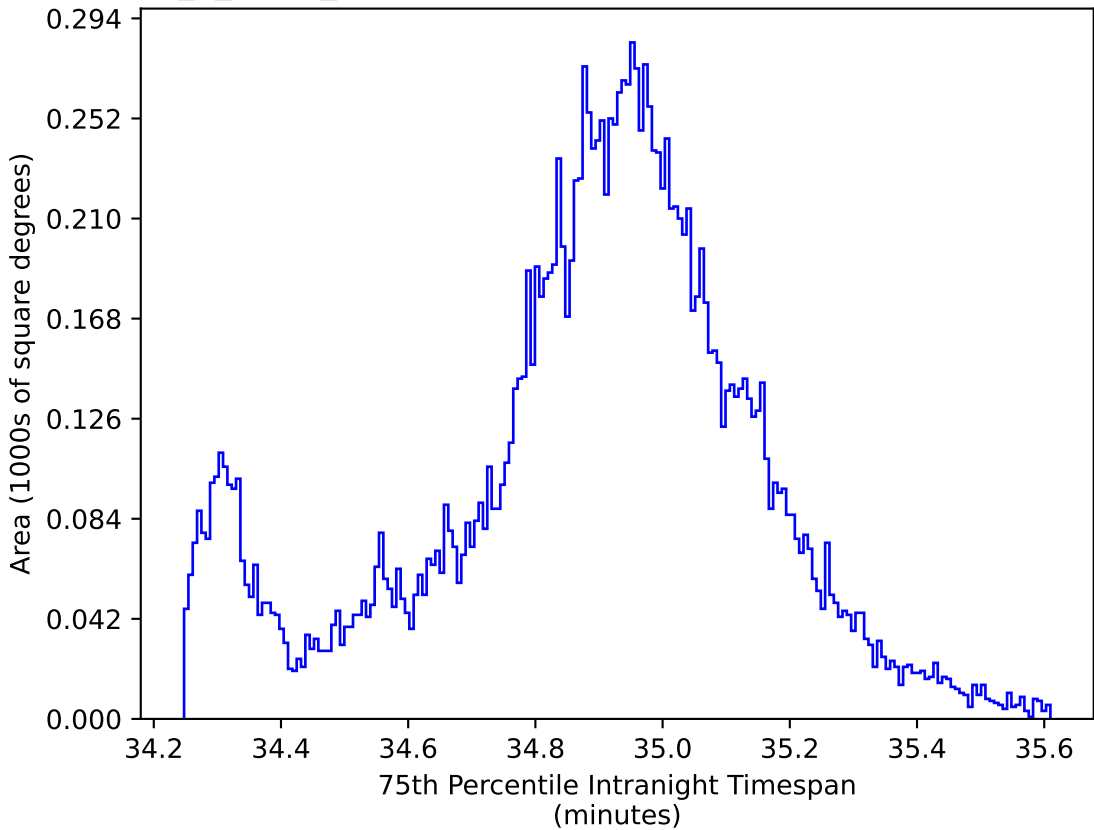
too_5_1v3.4_10yrs WFD: 75th Percentile Intranight Timespan
