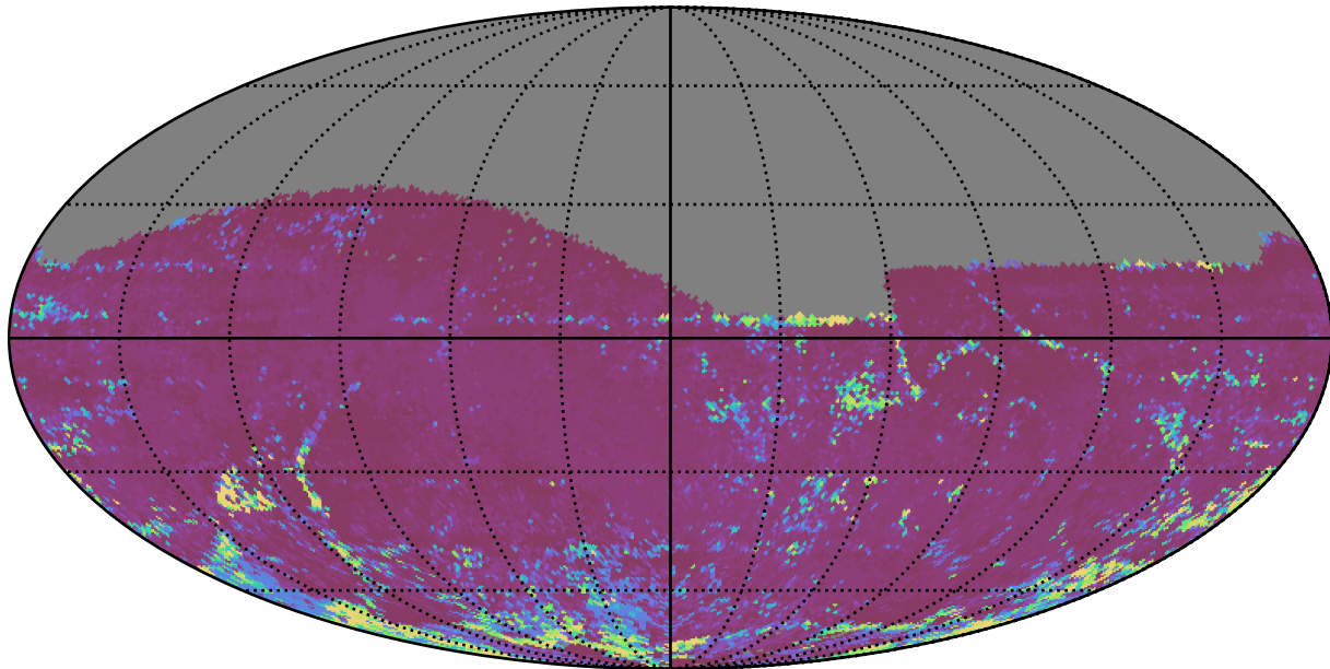
too_5_1v3.4_10yrs All sky z band: 75th Percentile Intranight Timespan
