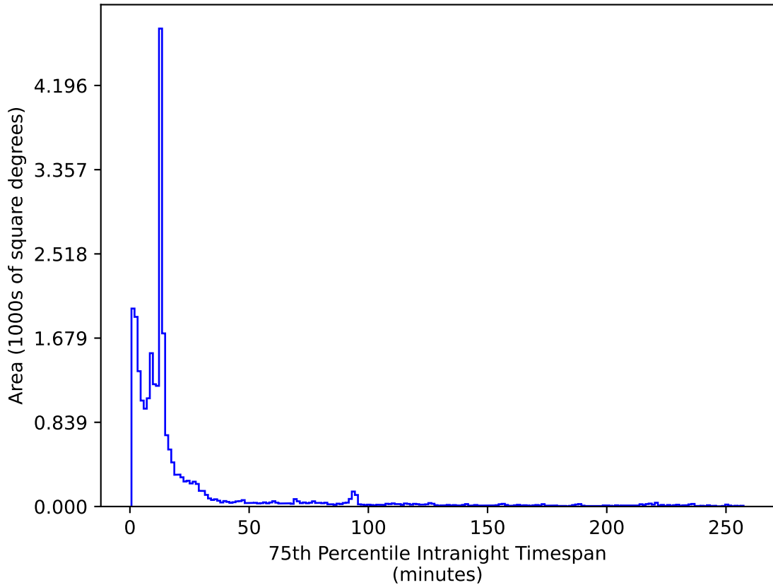
too_5_1v3.4_10yrs All sky z band: 75th Percentile Intranight Timespan
