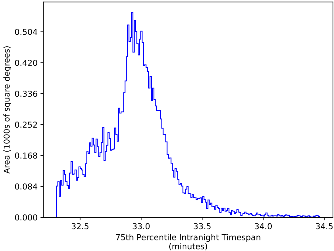
too_5_1v3.4_10yrs All sky y band: 75th Percentile Intranight Timespan
