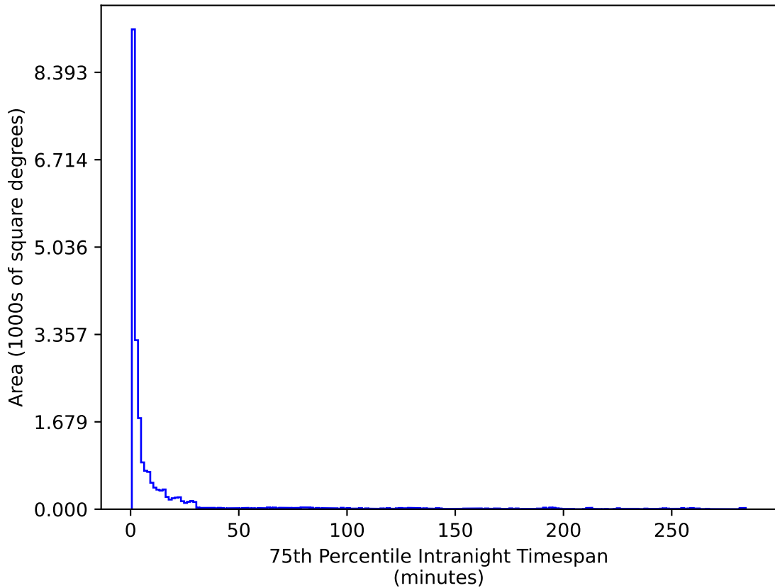
too_5_1v3.4_10yrs All sky u band: 75th Percentile Intranight Timespan
