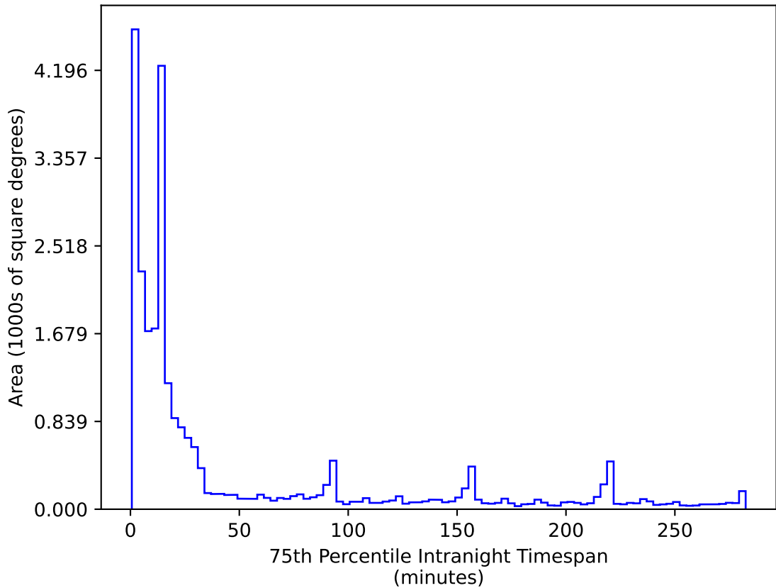
too_5_1v3.4_10yrs All sky r band: 75th Percentile Intranight Timespan
