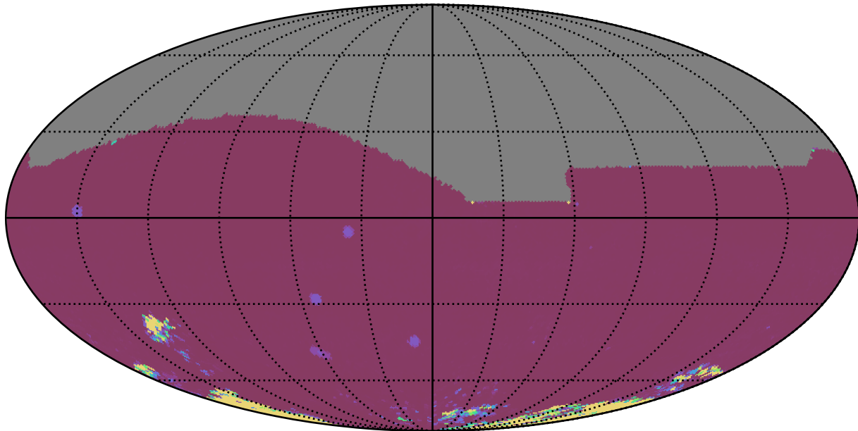
too_5_1v3.4_10yrs All sky iz bands: 75th Percentile Intranight Timespan
