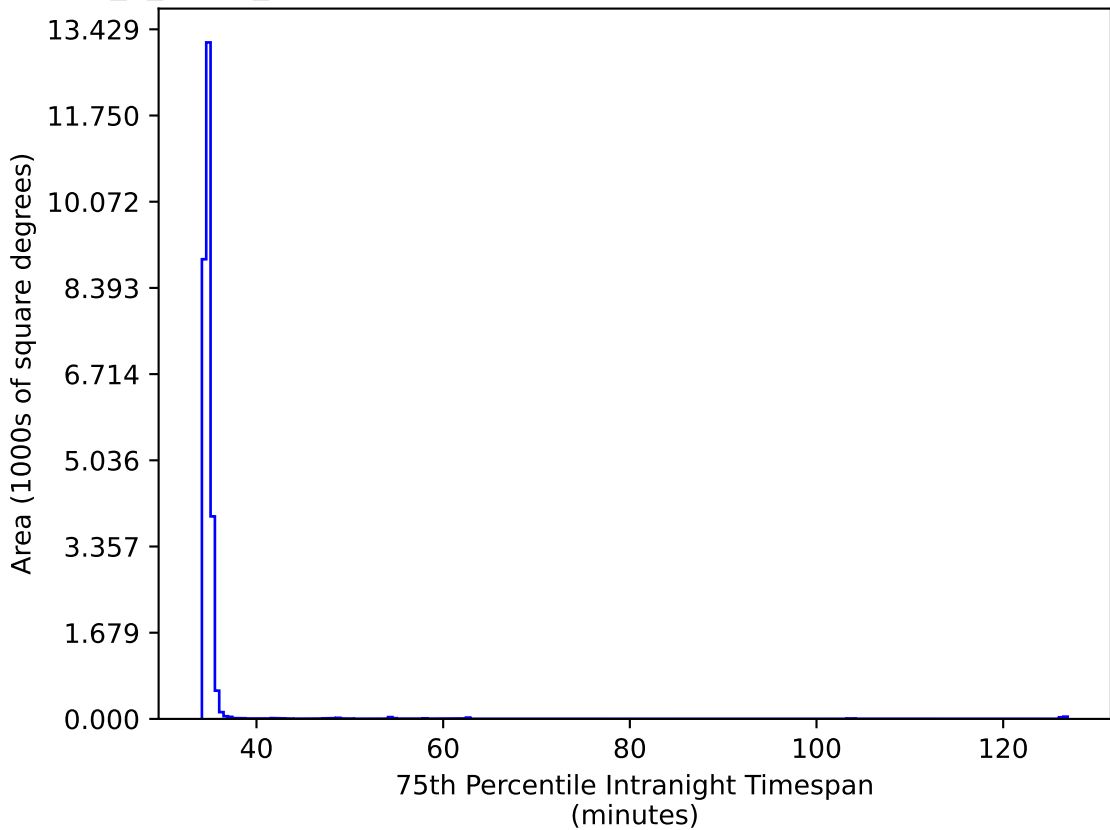
too_5_1v3.4_10yrs All sky iz bands: 75th Percentile Intranight Timespan
