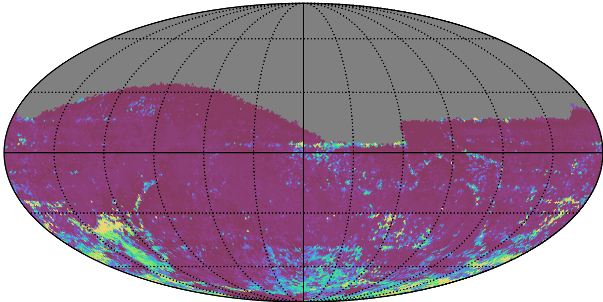
too_5_1v3.4_10yrs All sky i band: 75th Percentile Intranight Timespan
