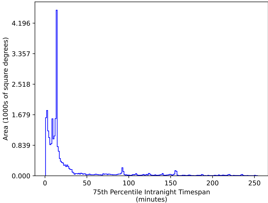
too_5_1v3.4_10yrs All sky i band: 75th Percentile Intranight Timespan
