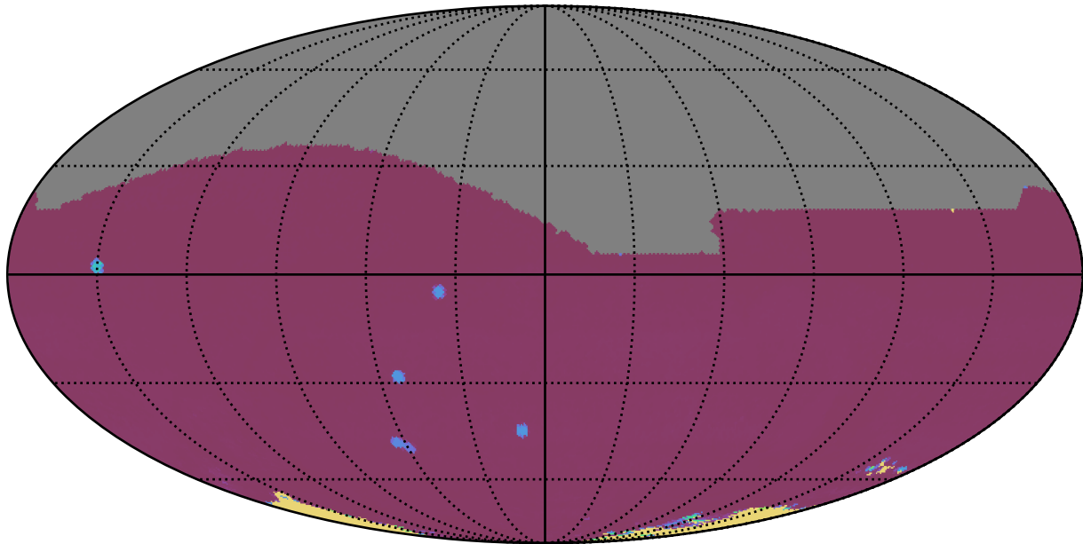
too_5_1v3.4_10yrs All sky: 75th Percentile Intranight Timespan
