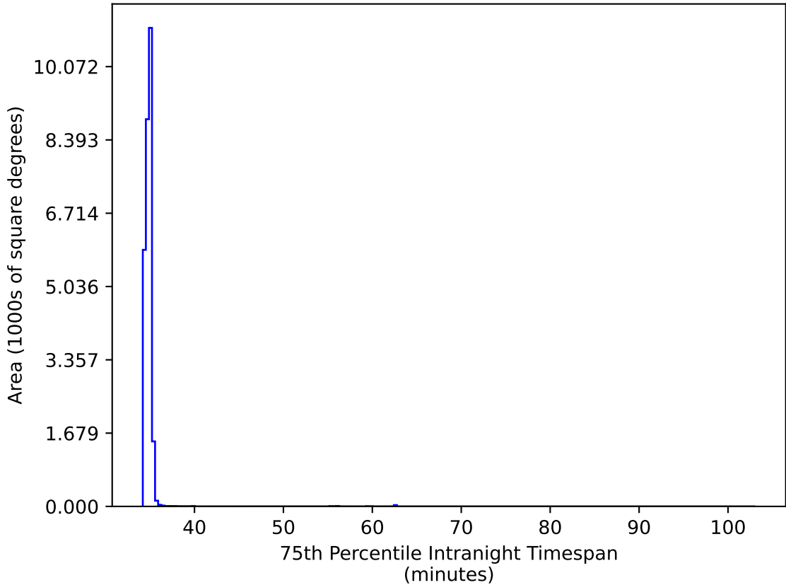
too_5_1v3.4_10yrs All sky: 75th Percentile Intranight Timespan
