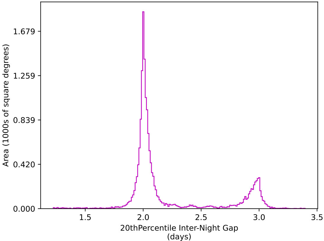
too_5_1v3.4_10yrs WFD z band: 20thPercentile Inter-Night Gap
