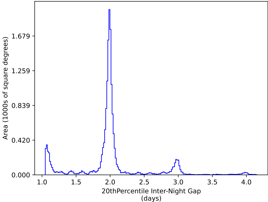
too_5_1v3.4_10yrs WFD y band: 20thPercentile Inter-Night Gap
