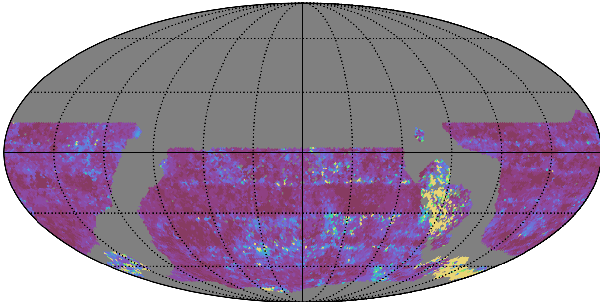
too_5_1v3.4_10yrs WFD u band: 20thPercentile Inter-Night Gap
