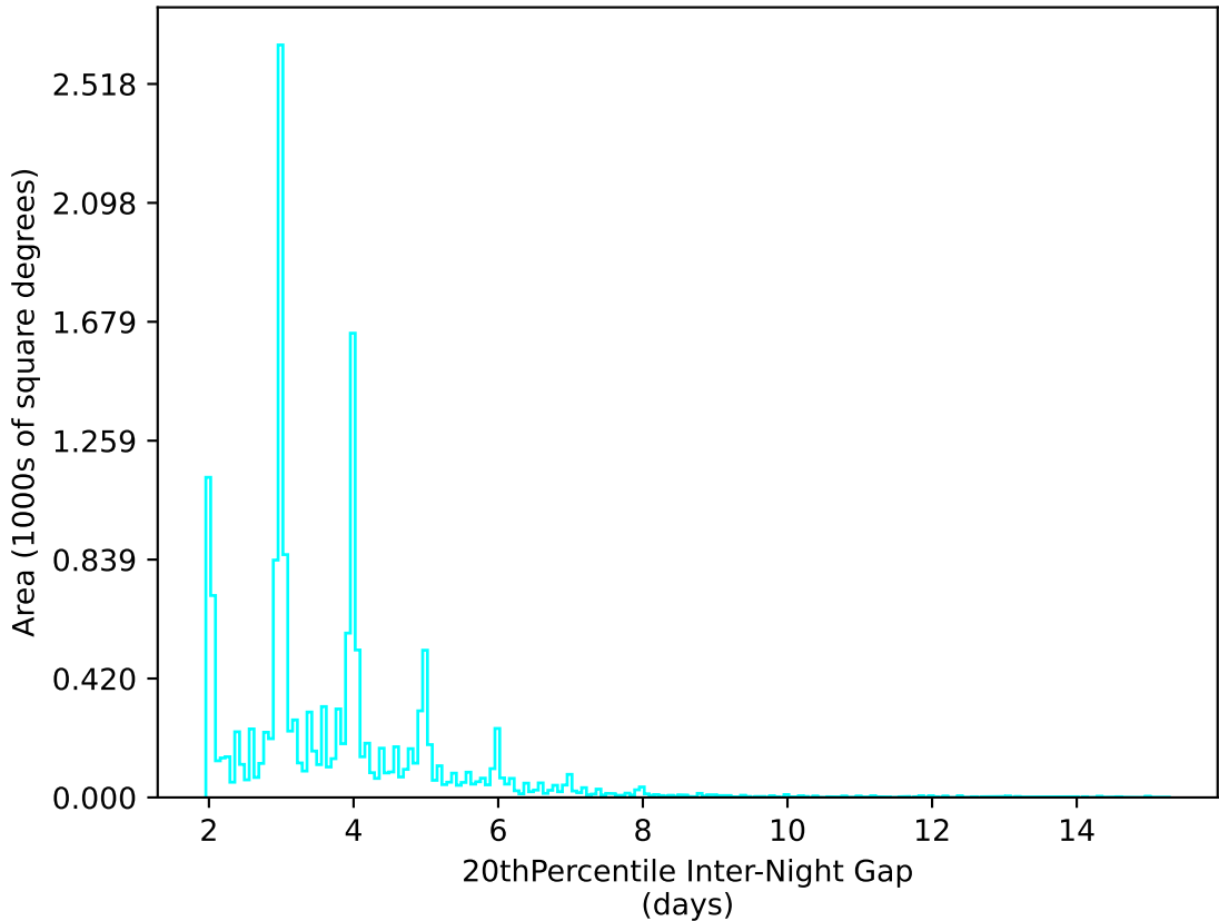
too_5_1v3.4_10yrs WFD u band: 20thPercentile Inter-Night Gap
