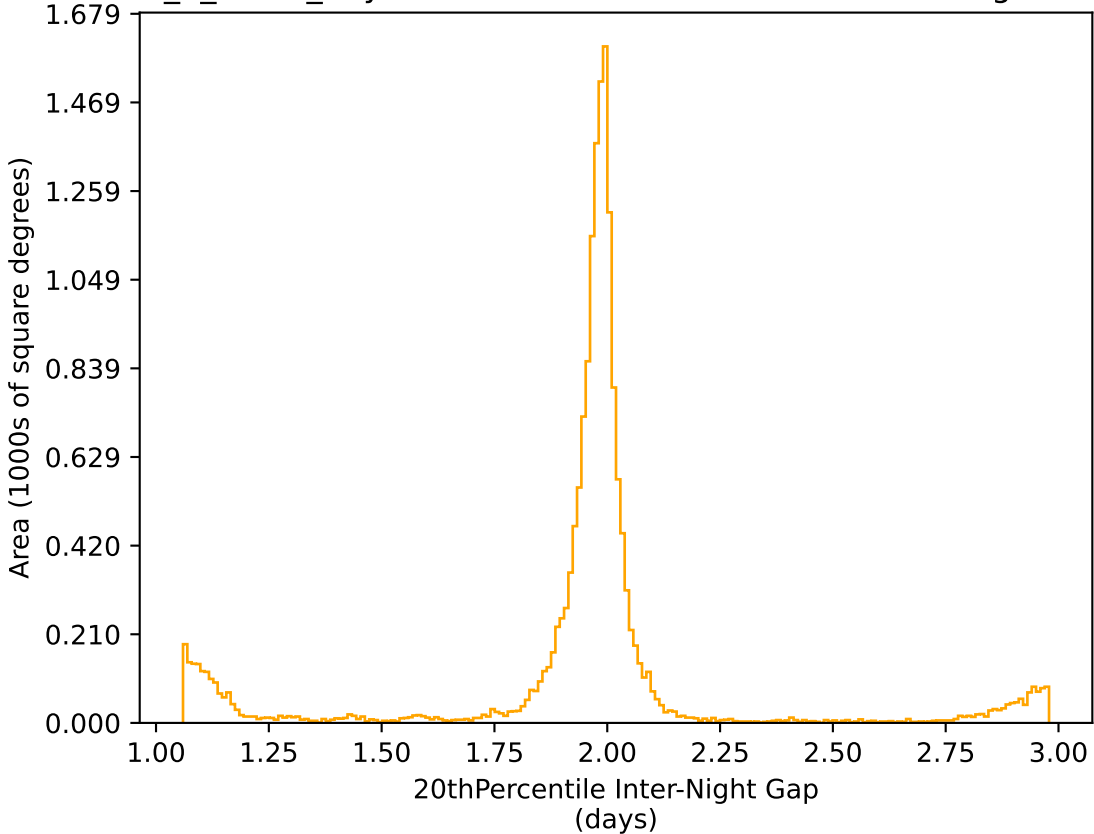
too_5_1v3.4_10yrs WFD r band: 20thPercentile Inter-Night Gap
