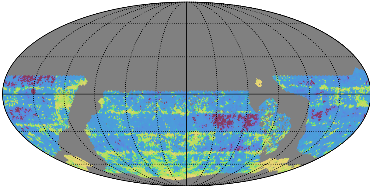
too_5_1v3.4_10yrs WFD i band: 20thPercentile Inter-Night Gap
