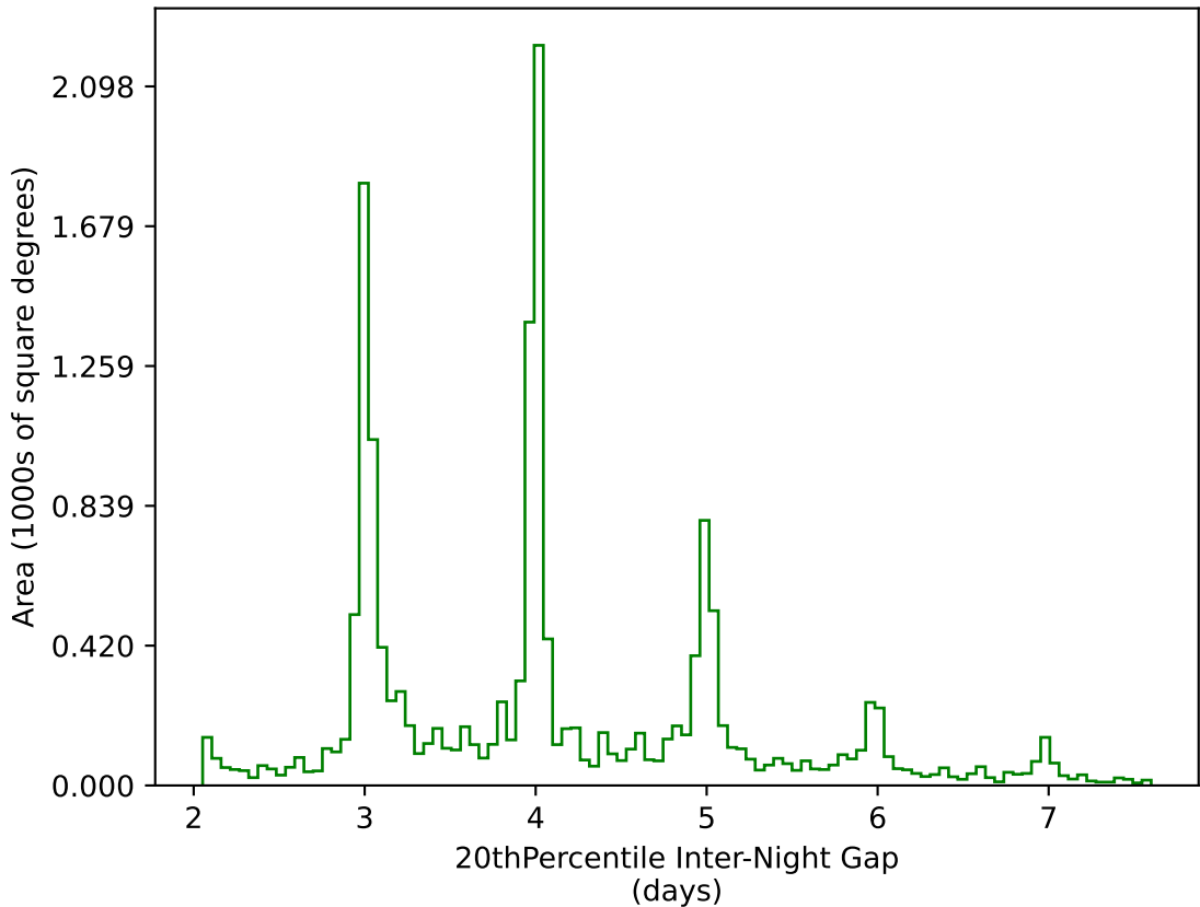
too_5_1v3.4_10yrs WFD g band: 20thPercentile Inter-Night Gap
