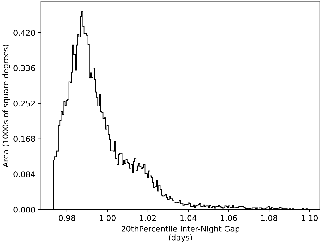
too_5_1v3.4_10yrs WFD all bands: 20thPercentile Inter-Night Gap
