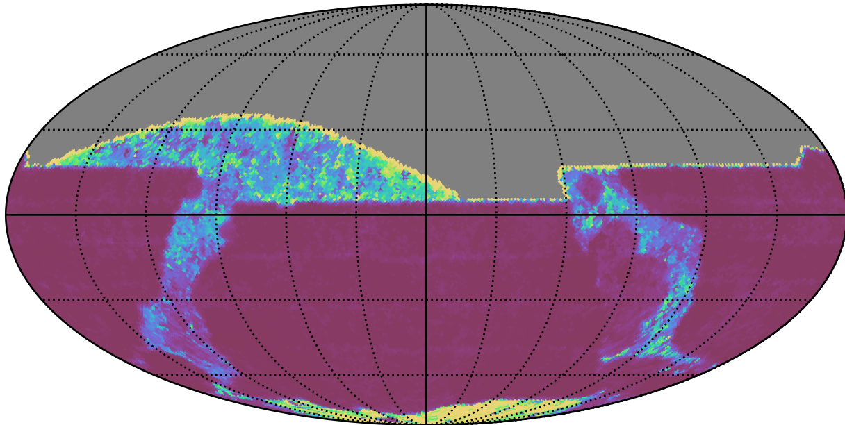
too_5_1v3.4_10yrs All sky z band: 20thPercentile Inter-Night Gap
