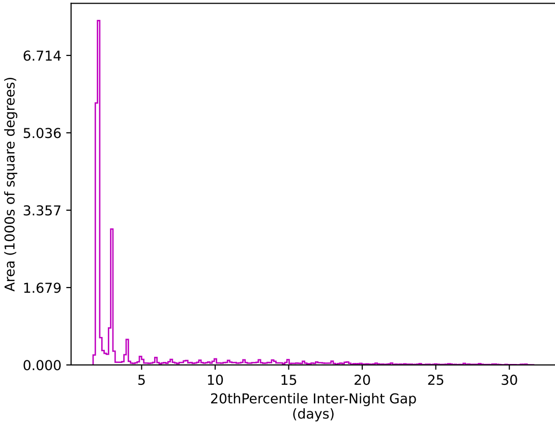
too_5_1v3.4_10yrs All sky z band: 20thPercentile Inter-Night Gap
