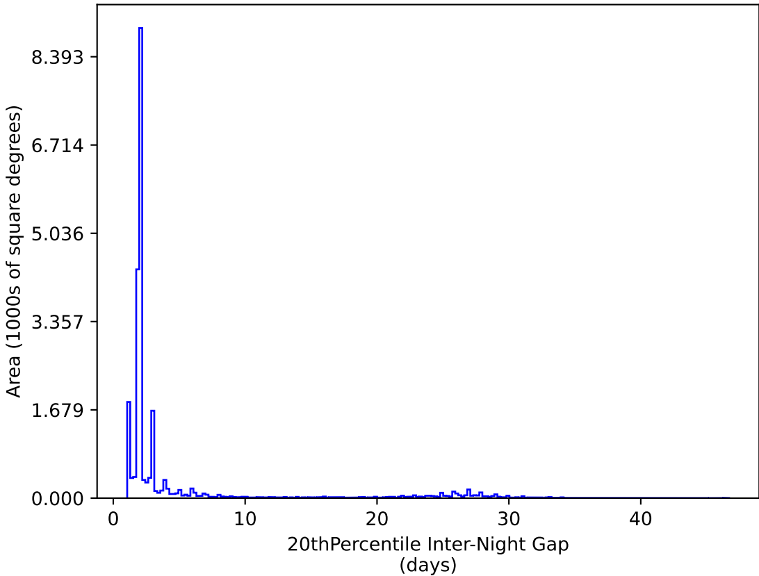
too_5_1v3.4_10yrs All sky y band: 20thPercentile Inter-Night Gap
