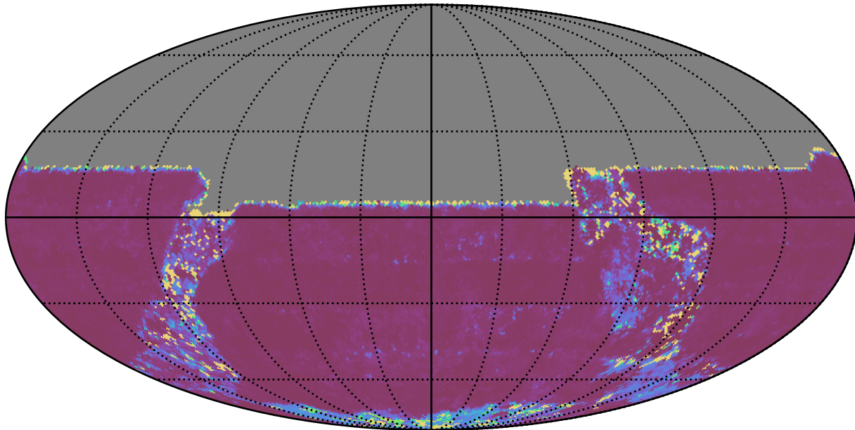
too_5_1v3.4_10yrs All sky u band: 20thPercentile Inter-Night Gap
