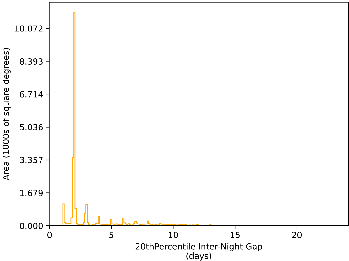
too_5_1v3.4_10yrs All sky r band: 20thPercentile Inter-Night Gap
