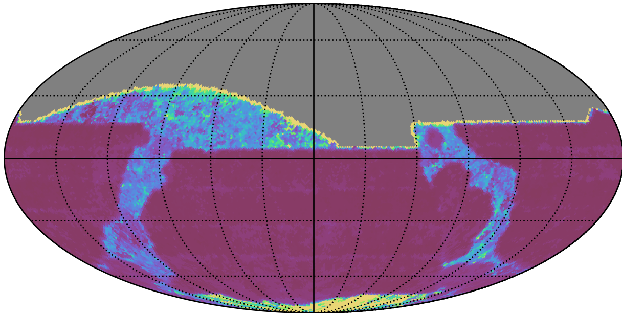
too_5_1v3.4_10yrs All sky i band: 20thPercentile Inter-Night Gap
