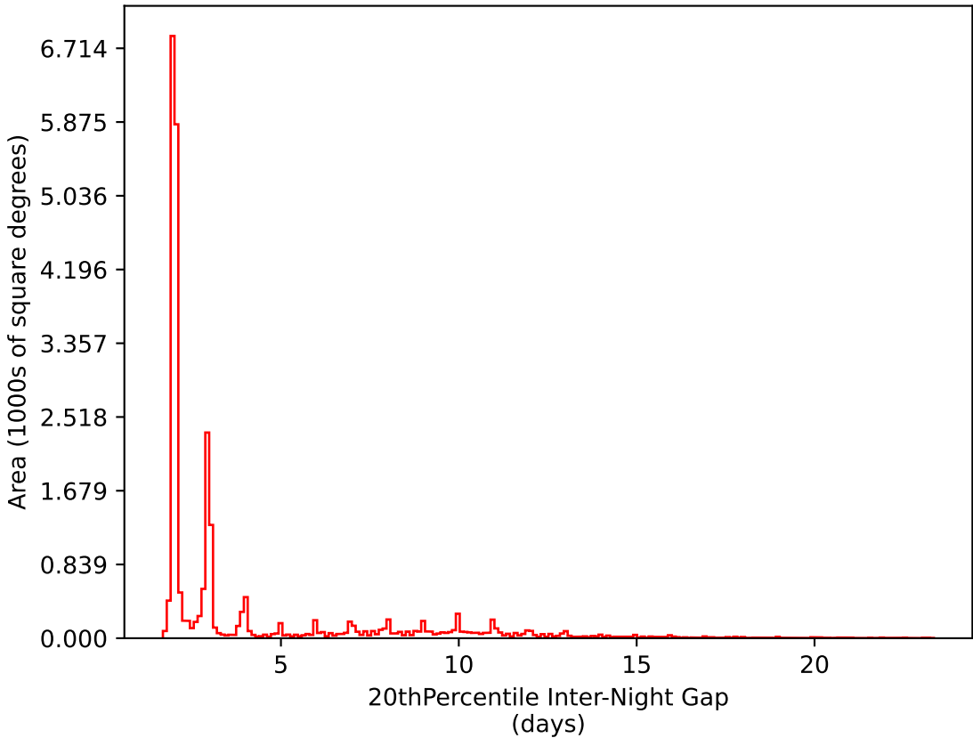
too_5_1v3.4_10yrs All sky i band: 20thPercentile Inter-Night Gap
