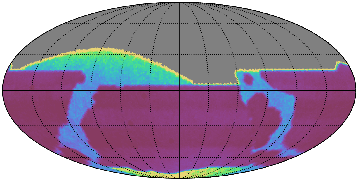
too_5_1v3.4_10yrs : properMotion
