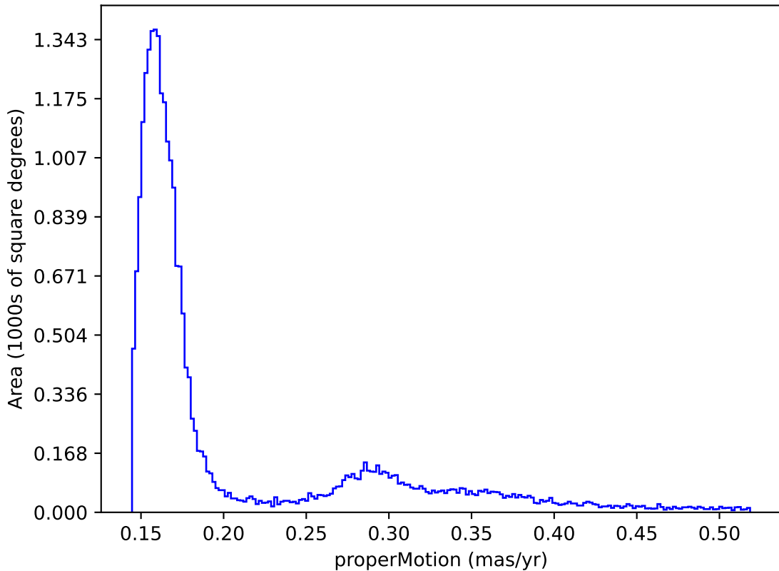
too_5_1v3.4_10yrs : properMotion
