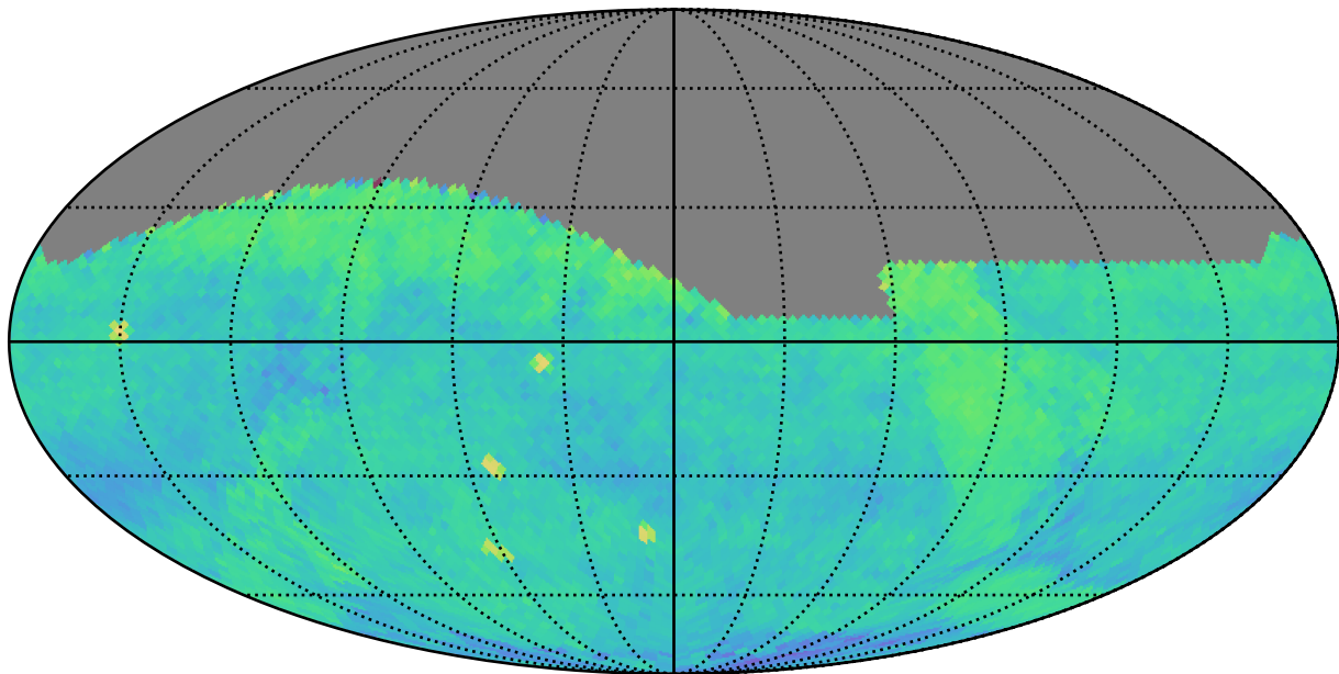
too_5_1v3.4_10yrs (g or r or i): PairFraction
