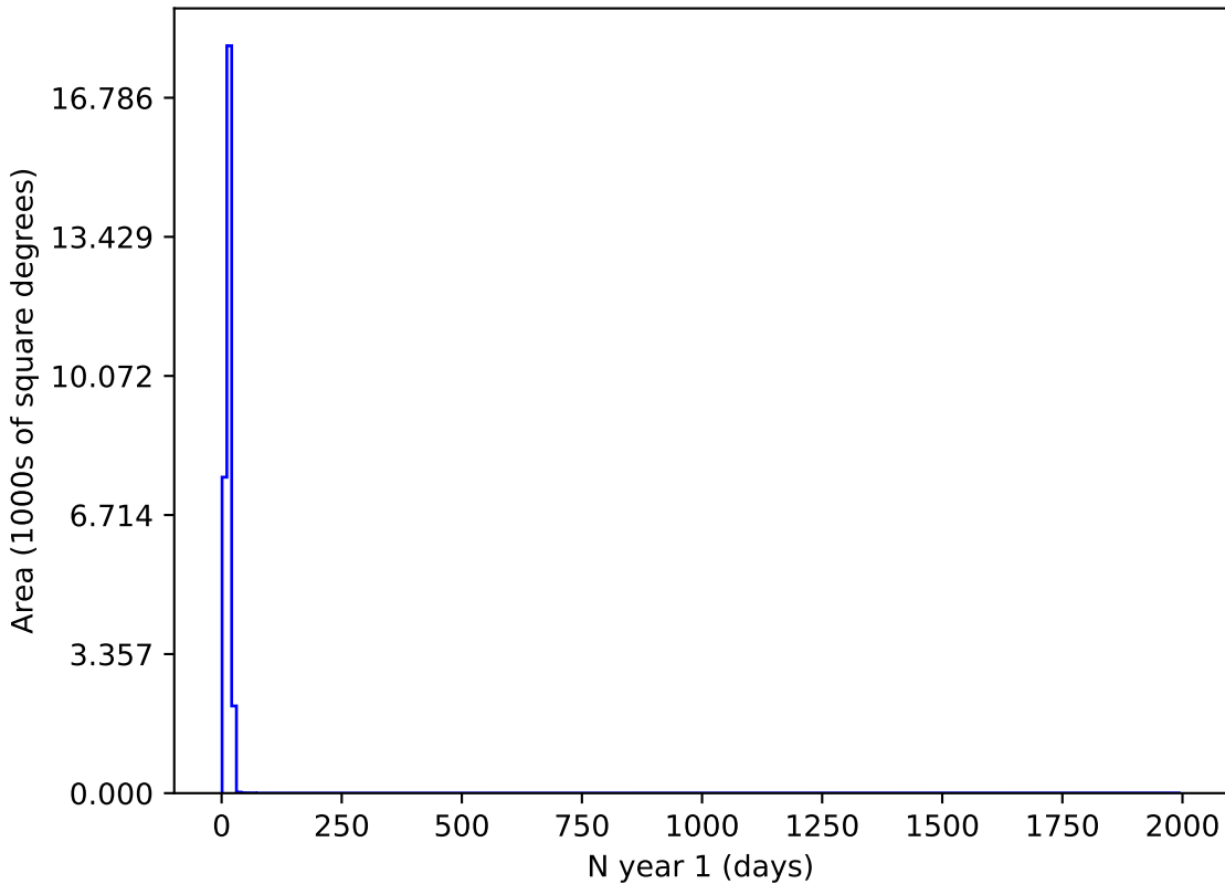
too_5_1v3.4_10yrs z and night < 365: N year 1
