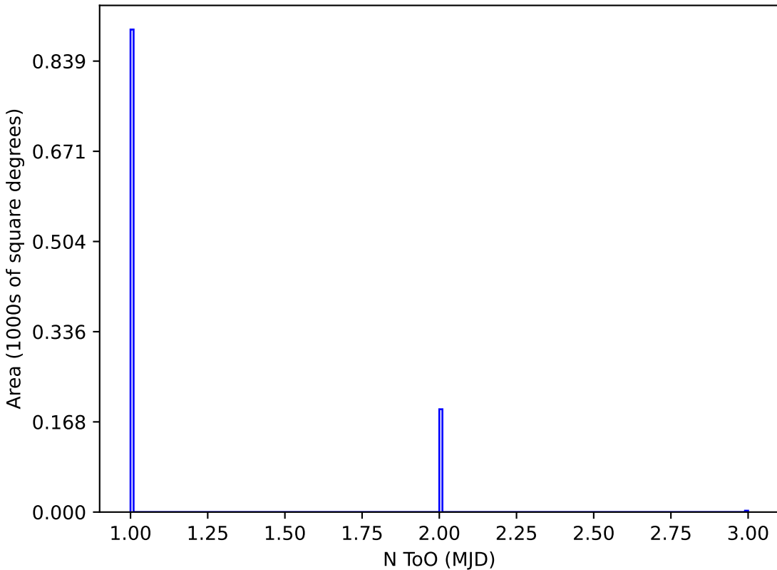
too_5_1v3.4_10yrs z and note like ToO%: N ToO
