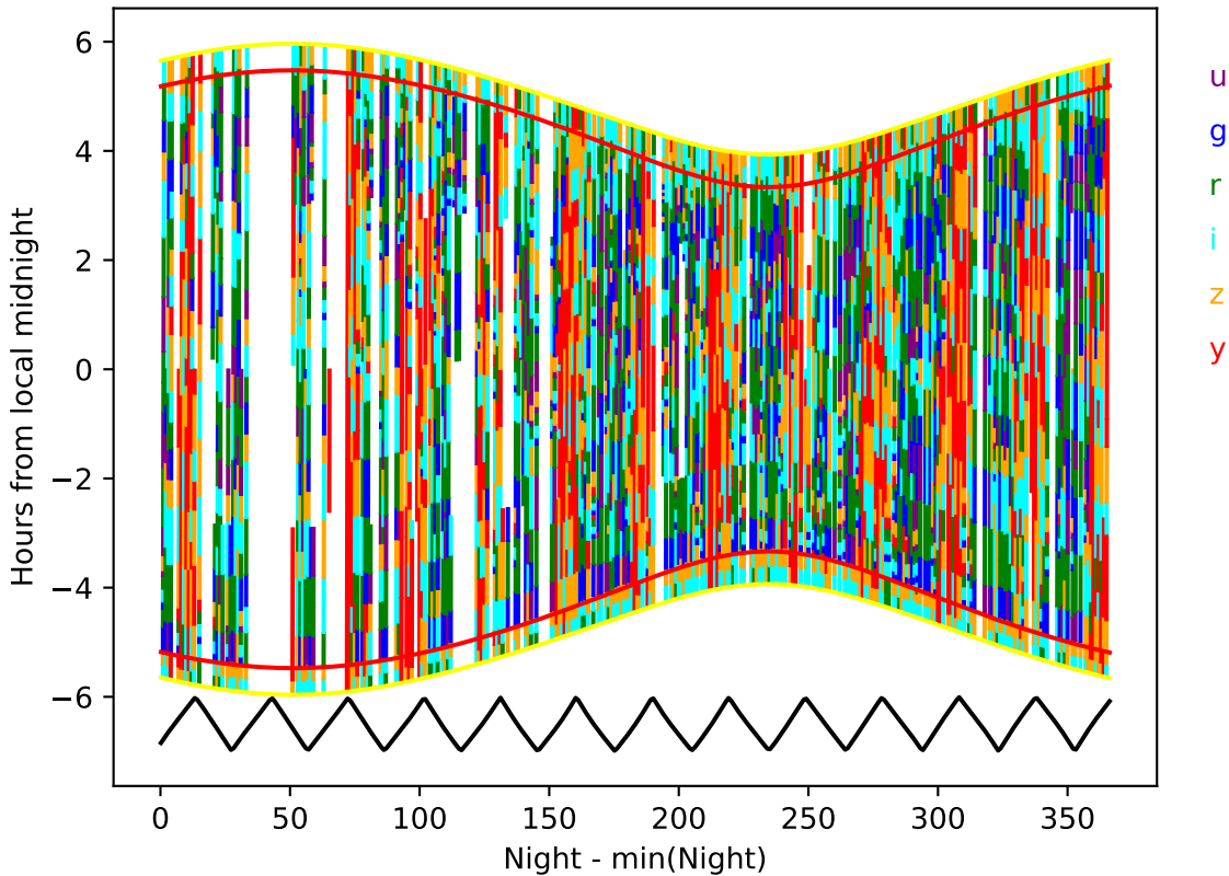
too_5_1v3.4_10yrs year 8-9: Hourglass
