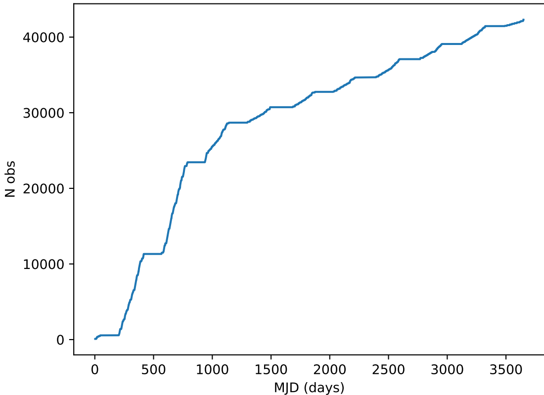
too_5_1v3.4_10yrs note like DD:COSMOS%: Cumulative
