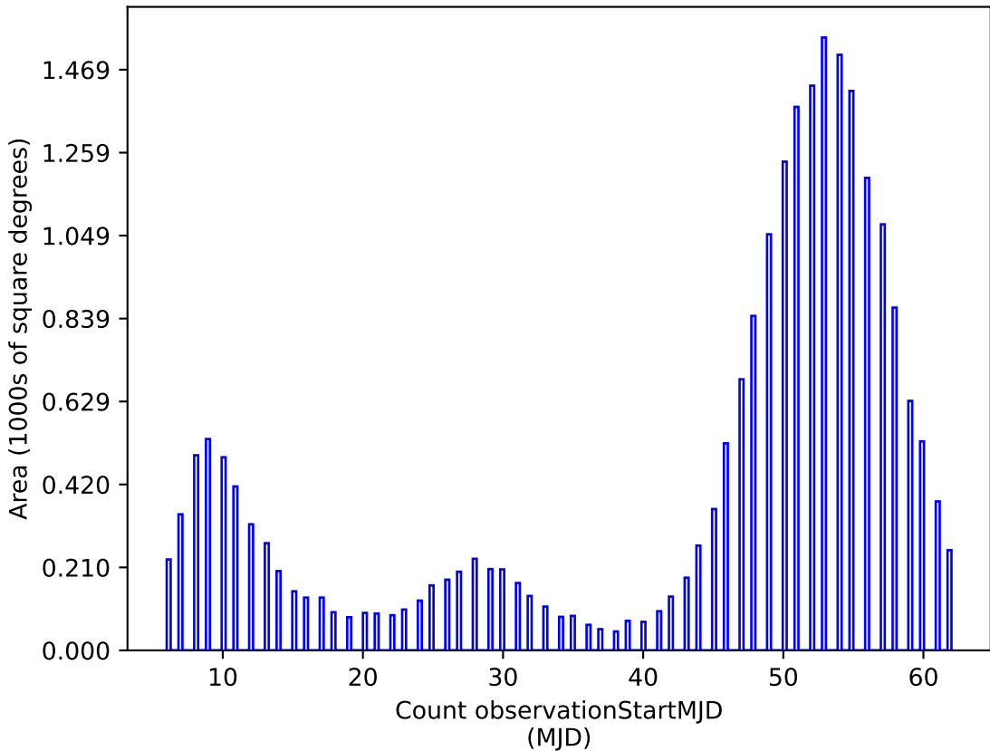
too_5_1v3.4_10yrs u: Count observationStartMJD
