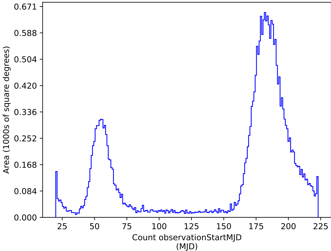
too_5_1v3.4_10yrs r: Count observationStartMJD
