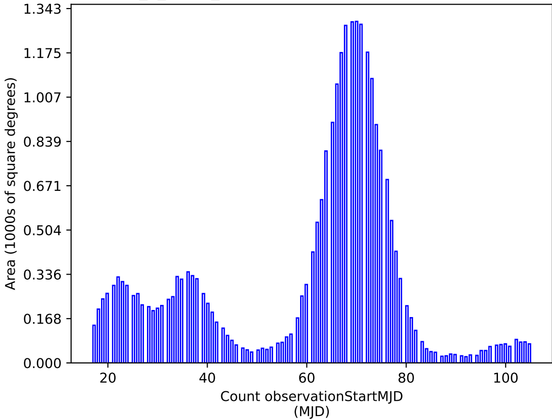
too_5_1v3.4_10yrs g: Count observationStartMJD
