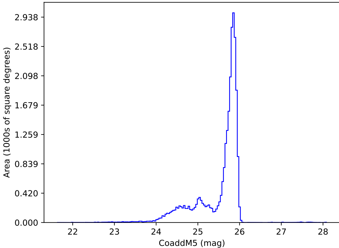
too_5_1v3.4_10yrs z: CoaddM5
