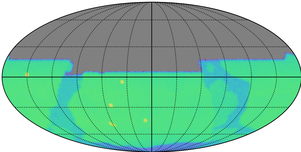
too_5_1v3.4_10yrs y: CoaddM5
