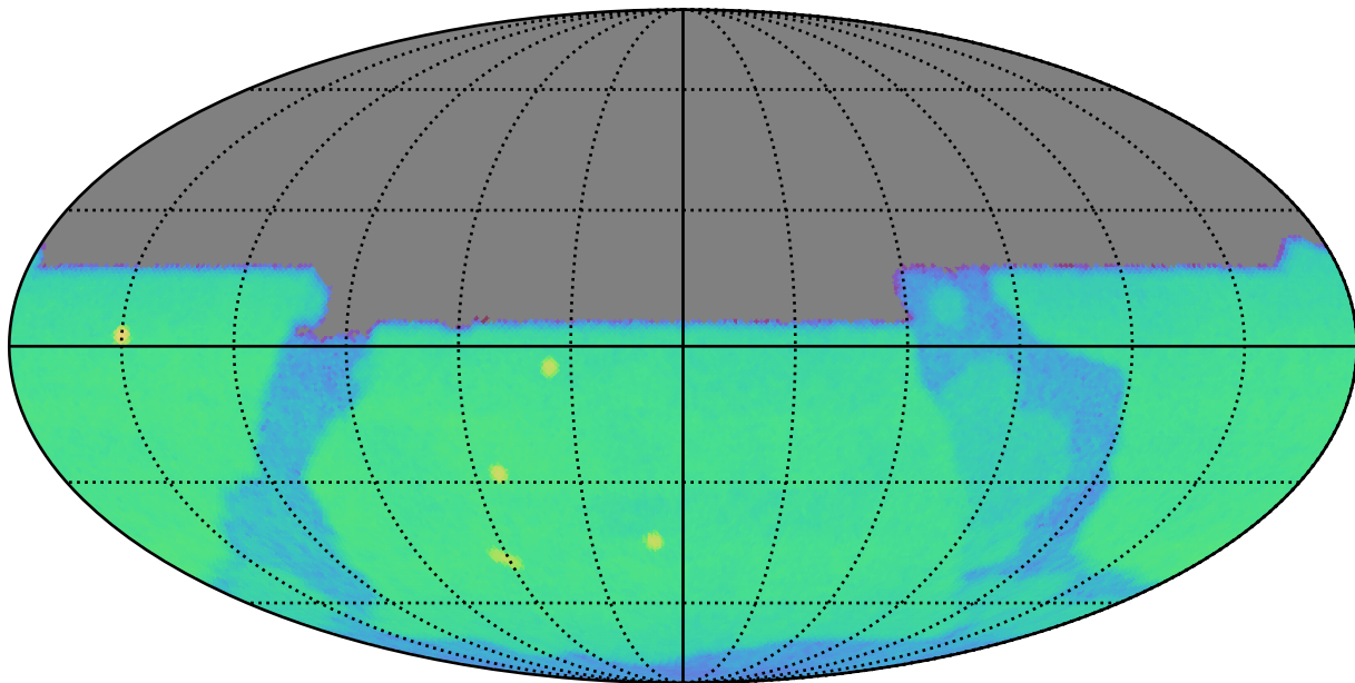
too_5_1v3.4_10yrs u: CoaddM5
