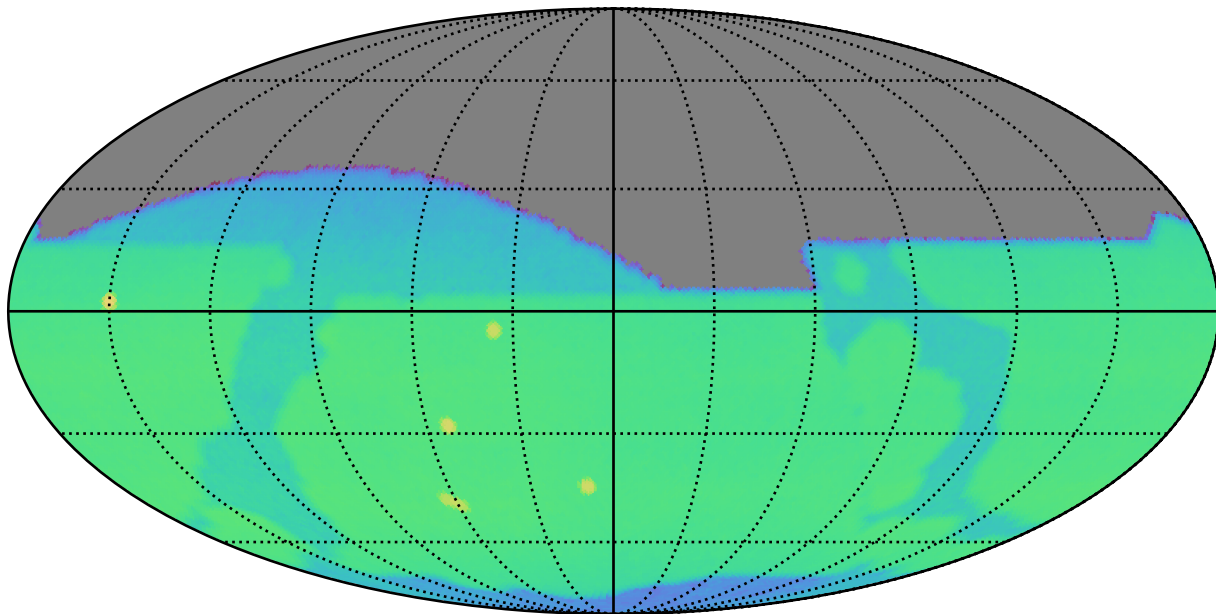
too_5_1v3.4_10yrs r: CoaddM5
